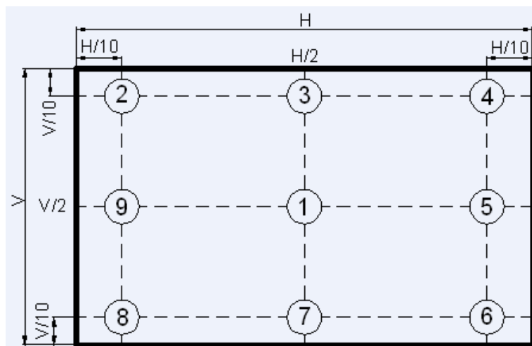
Figure 6 Measurement Locations
